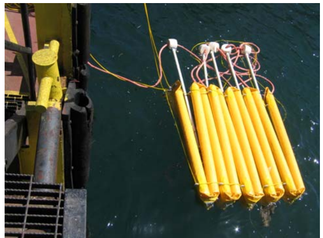
Compacts in-the-water for Re-deployment and Recovery
