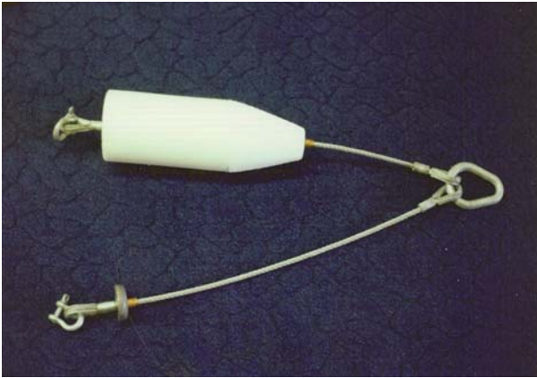
TOW BRIDLE ASSEMBLY: This system is designed for a stable two-point tow load and includes a heavy duty pear link, high test steel cables, float, ballast and steel shackles.
